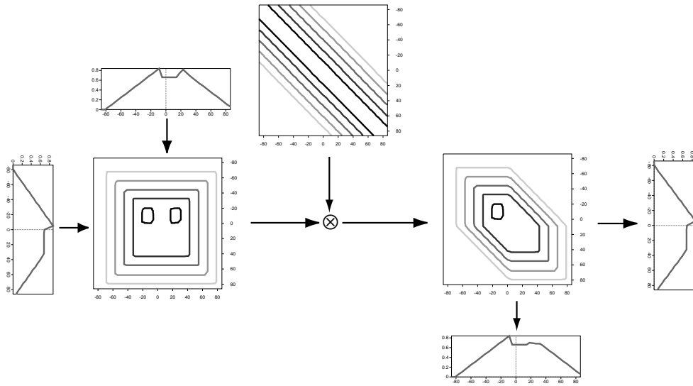
Figure 2: Computation of Joint and Marginal Desirability Functions
