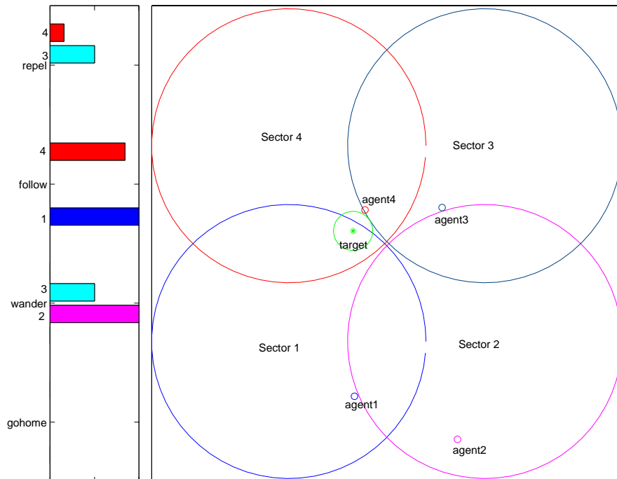
Figure 4: Multiple agents covering a target
