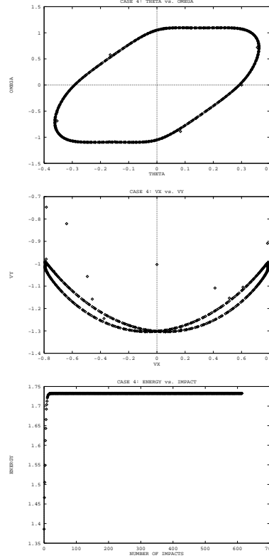
Figure 4: Example without noise: \theta_0 = 0.3 rad., e = 0.5 , \kappa = 1.1 , \kappa_E = 0.165 , \eta^* = 1.73
